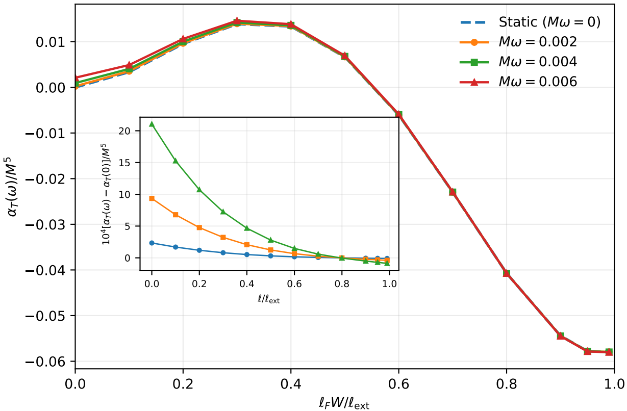
Tensor-probe response on the Fan-Wang background
