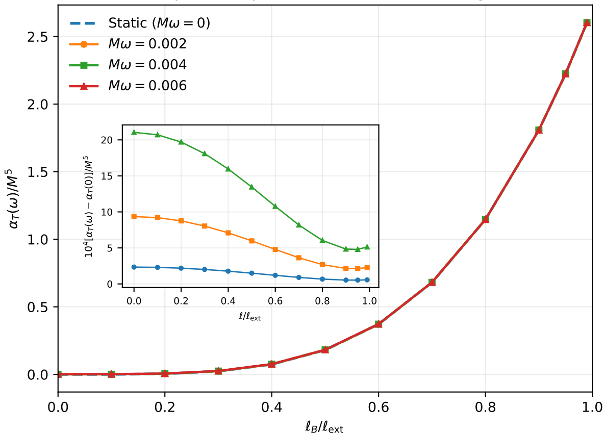
Tensor-probe response on the Bardeen background
