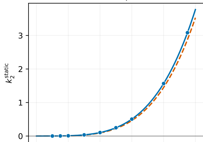
Bardeen polar
