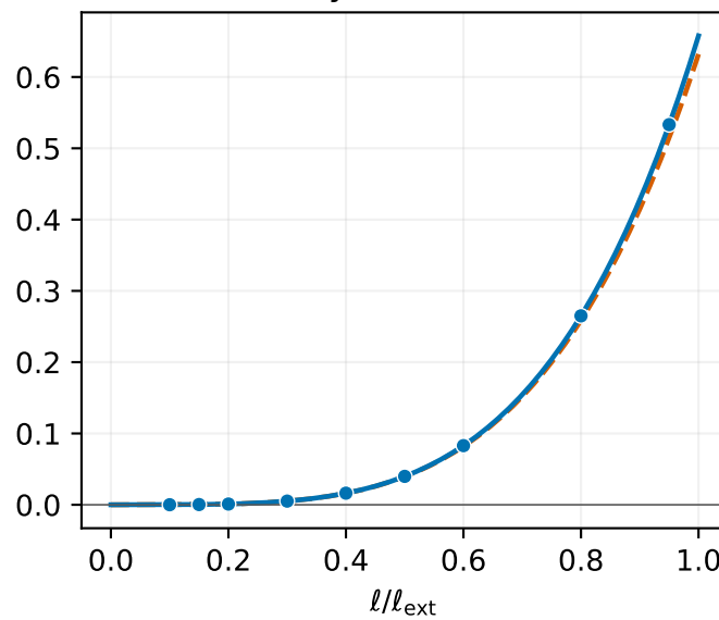
Hayward axial
