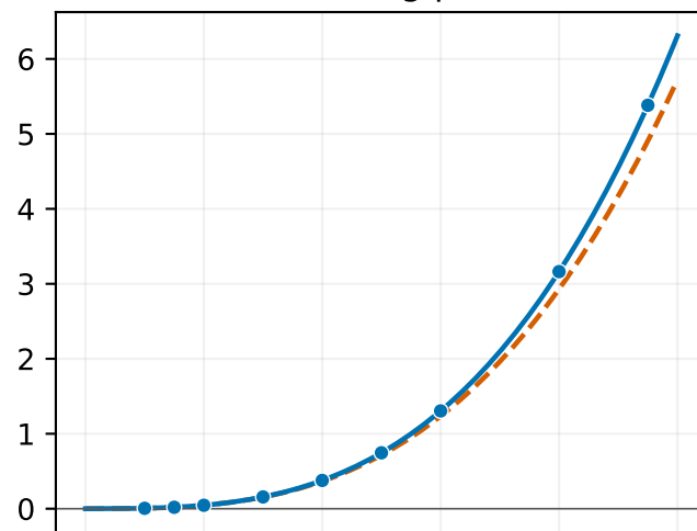
Fan--Wang polar
