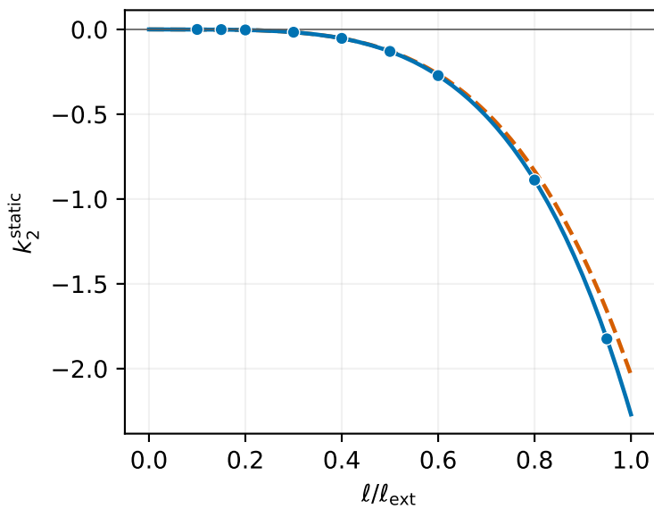
Bardeen axial
