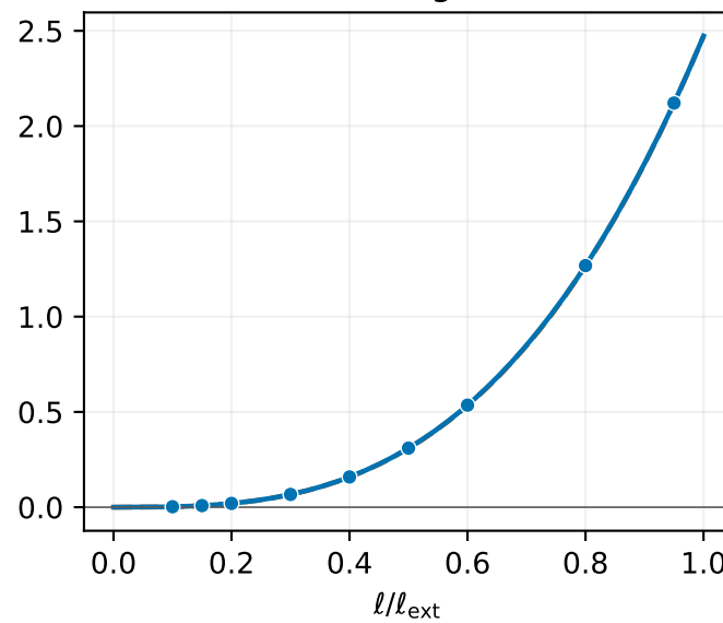
Fan--Wang axial
