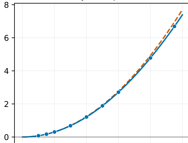
Hayward polar
