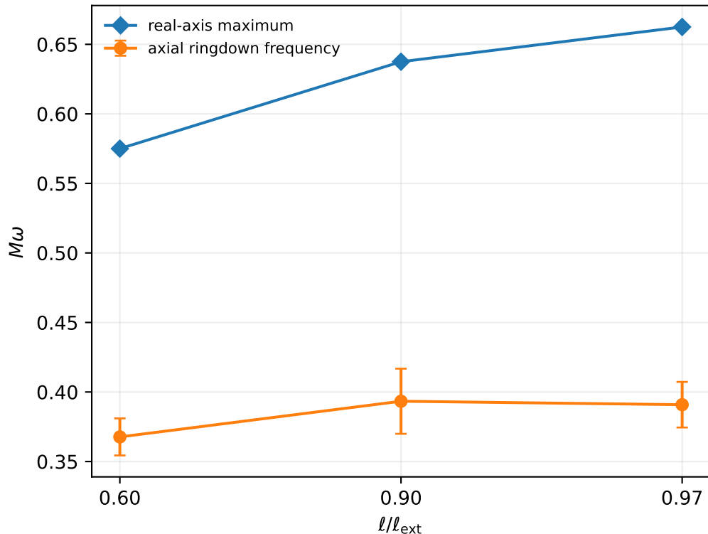
QNM-resonance alignment
