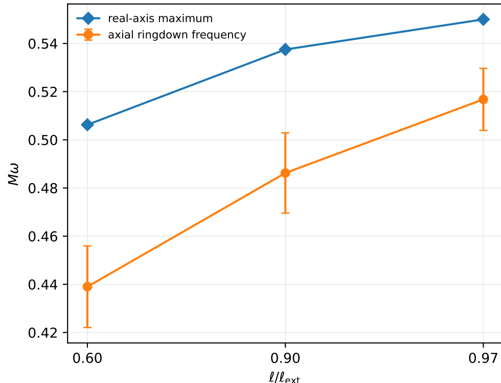
QNM-resonance alignment
