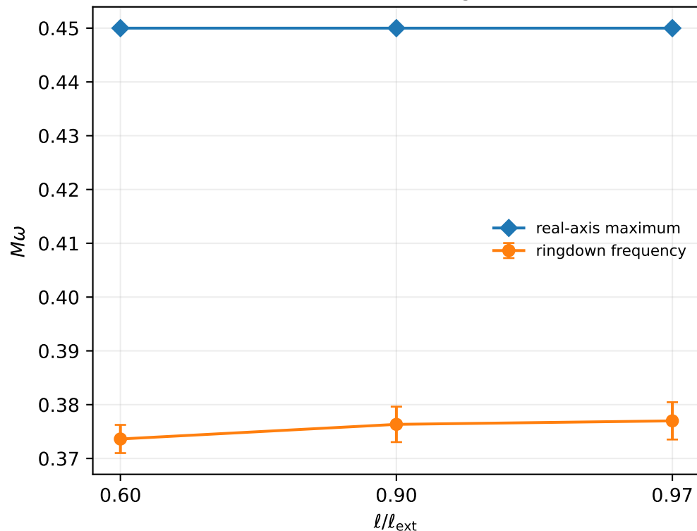
QNM-resonance alignment
