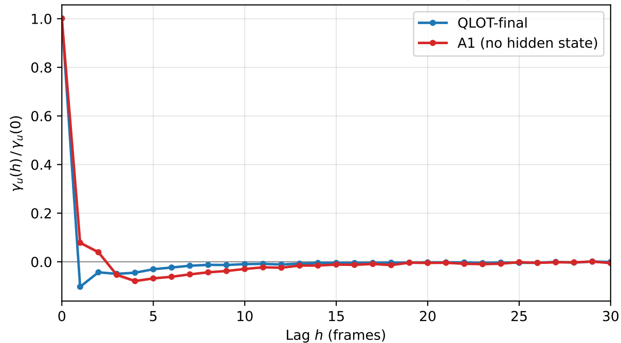
Delta-Error Autocorrelation (150 WFLW-V clips, 3 seeds)
