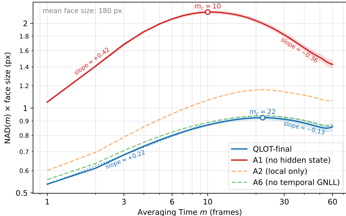
Normalized Allan Deviation (150 WFLW-V clips, 3 seeds)
