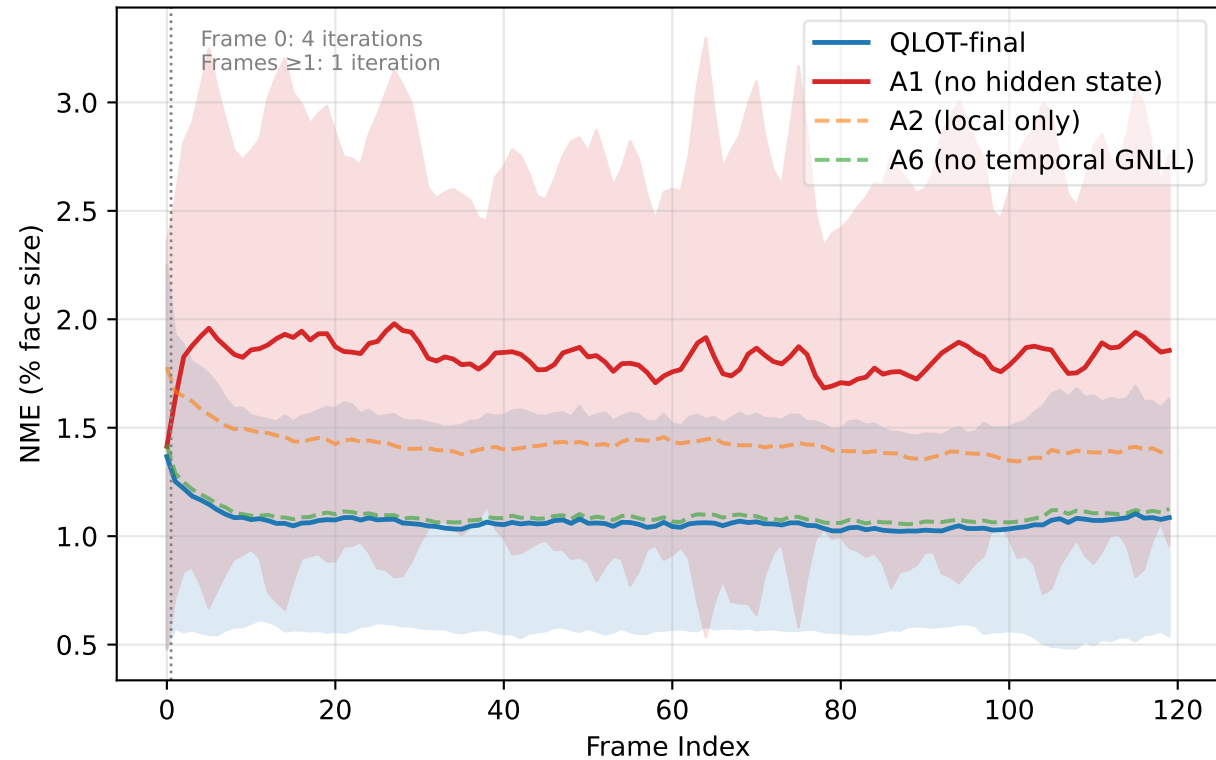
Per-frame Tracking Error (150 WFLW-V clips, 3 seeds)
