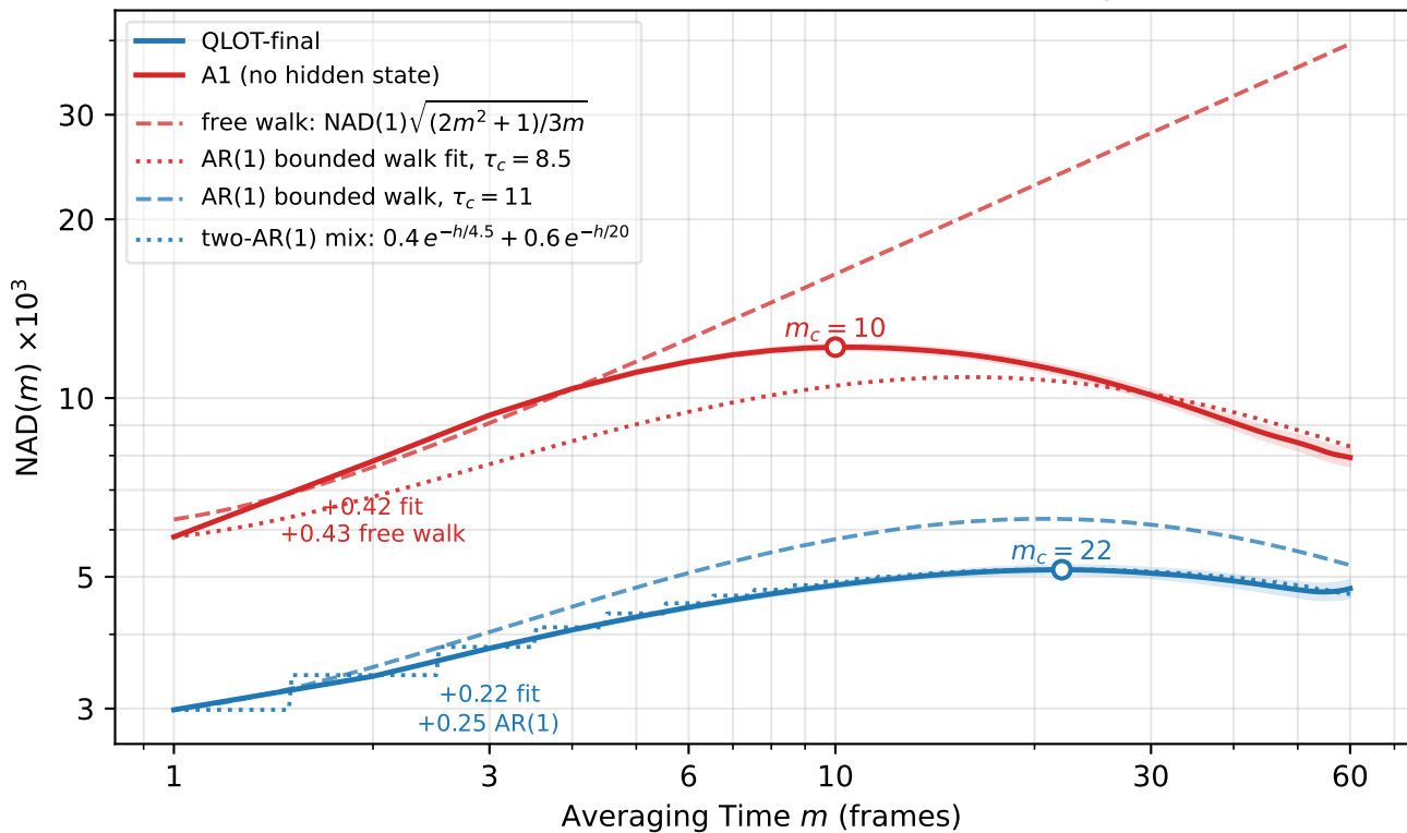
NAD vs. Canonical Error Processes (150 WFLW-V clips, 3 seeds)
