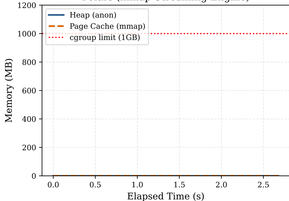
Polars (mmap Streaming Engine)
