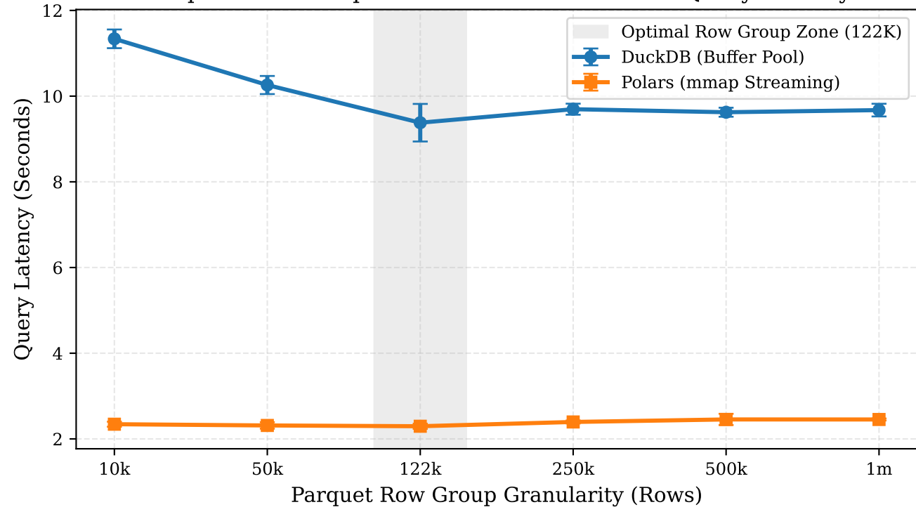
Parquet Row-Group Continuum vs Out-Of-Core Query Latency
