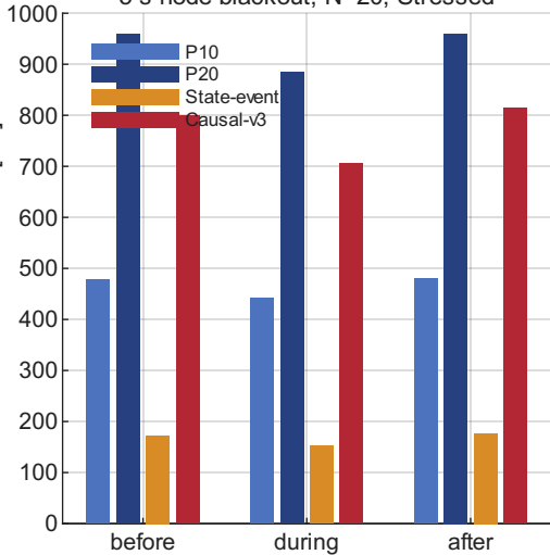
5 s node blackout, N=20, Stressed
