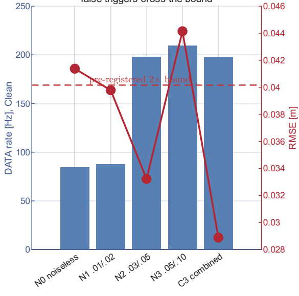
Estimator noise buys traffic, not accuracy: false triggers cross the bound
