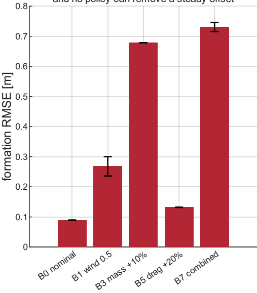
Plant mismatch: the mass arm dominates, and no policy can remove a steady offset
