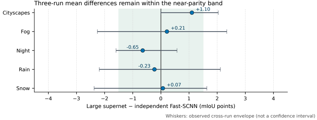
Figure 5: Three-run matched-capacity comparison. Points are differences between the mean mIoU of the large elastic candidate and independently trained Fast-SCNN; positive values favor the elastic candidate. Whiskers show the full observed cross-run envelope formed from the two three-run sets and are descriptive, not confidence intervals or paired-seed estimates. Every observed mean remains inside the prespecified \pm 1.5 -point practical near-parity band; this does not establish superiority or statistical equivalence.
