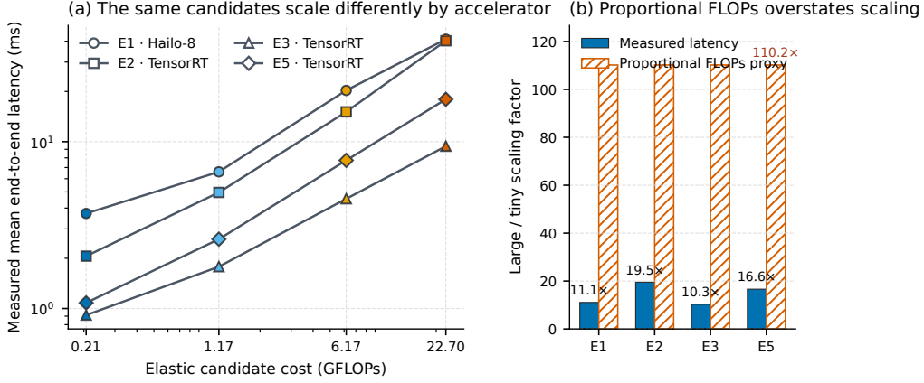
Figure 4: Why FLOPs is insufficient as a deployment-cost proxy. (a) The four elastic levels are plotted at their actual GFLOPs and measured mean end-to-end latency on E1, E2, E3, and E5; marker shape identifies hardware and marker color identifies capacity. (b) Large increases compute by 110.2 \times relative to tiny, but measured latency increases by only 10.3–19.5 \times , depending on the accelerator. FLOPs preserves the candidate order here but not the hardware-specific cost scale required by a latency budget.
