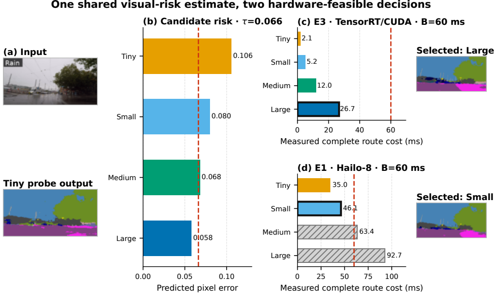
Figure 6: Hardware-cost-conditioned routing for one audited held-out rain image. (a) The input and tiny probe output are cropped without alteration from the deterministic qualitative artifact. (b) One probe score maps to four candidate-specific predicted errors; the dashed line is the configured target \tau = 0.066 . (c) With an illustrative B = 60 ms budget, every measured E3 warm route is feasible and large is selected. (d) Under the same budget on E1, medium and large are infeasible (hatched), so small is selected. The example demonstrates the policy mechanism and does not add an independent evaluation trial.
