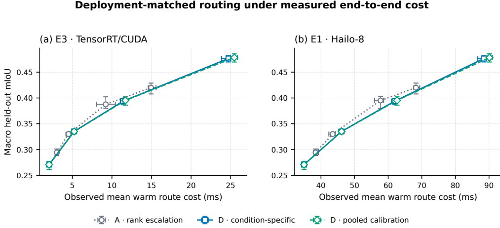
Figure 7: Quality versus measured complete warm-route cost after deployment-matched calibration. Each point first macro-averages the five held-out splits within one training run and then averages Runs A–C; horizontal and vertical whiskers show the full run-level range, not confidence intervals. Points are placed at observed mean route cost rather than nominal budget. Both candidate-specific hard-budget variants extend to higher-quality operating points than rank policy A; pooled calibration closely tracks configured condition-specific calibration on E3 and E1.
