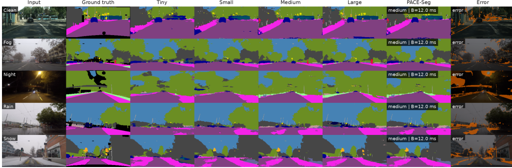
Figure 8: Qualitative capacity comparison on the five held-out examples from Fig. 3. Columns show input, ground truth, the four elastic candidates, configured PACE-Seg policy D, and an error overlay; orange marks disagreement between the selected output and ground truth. At the displayed E3 budget ( B = 11.97 ms), D selects medium for all five examples, so the PACE-Seg column intentionally matches Medium. Selection was fixed by median large-candidate pixel error before visual inspection, rather than by perceived success.
