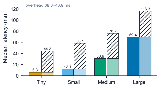
static deployment S (left) / route through tiny C (right) routing overhead C - S E3 AGX Xavier (TensorRT FP16) E1 Hailo-8 (INT8)
