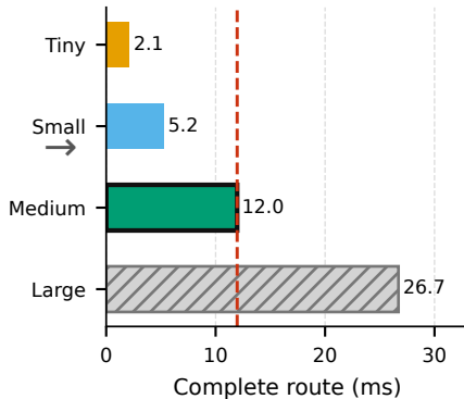
(e) E3 feasibility ( B=11.97 ms)
