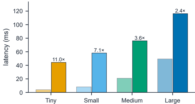
candidate-only p95 (left) complete-route median (right) AGX Xavier (TensorRT FP16) Hailo-8 (INT8)
