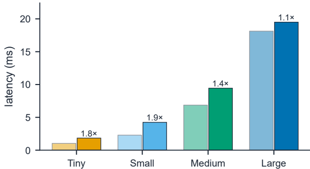
candidate-only p95 (left) complete-route median (right) AGX Xavier (TensorRT FP16) Hailo-8 (INT8)
