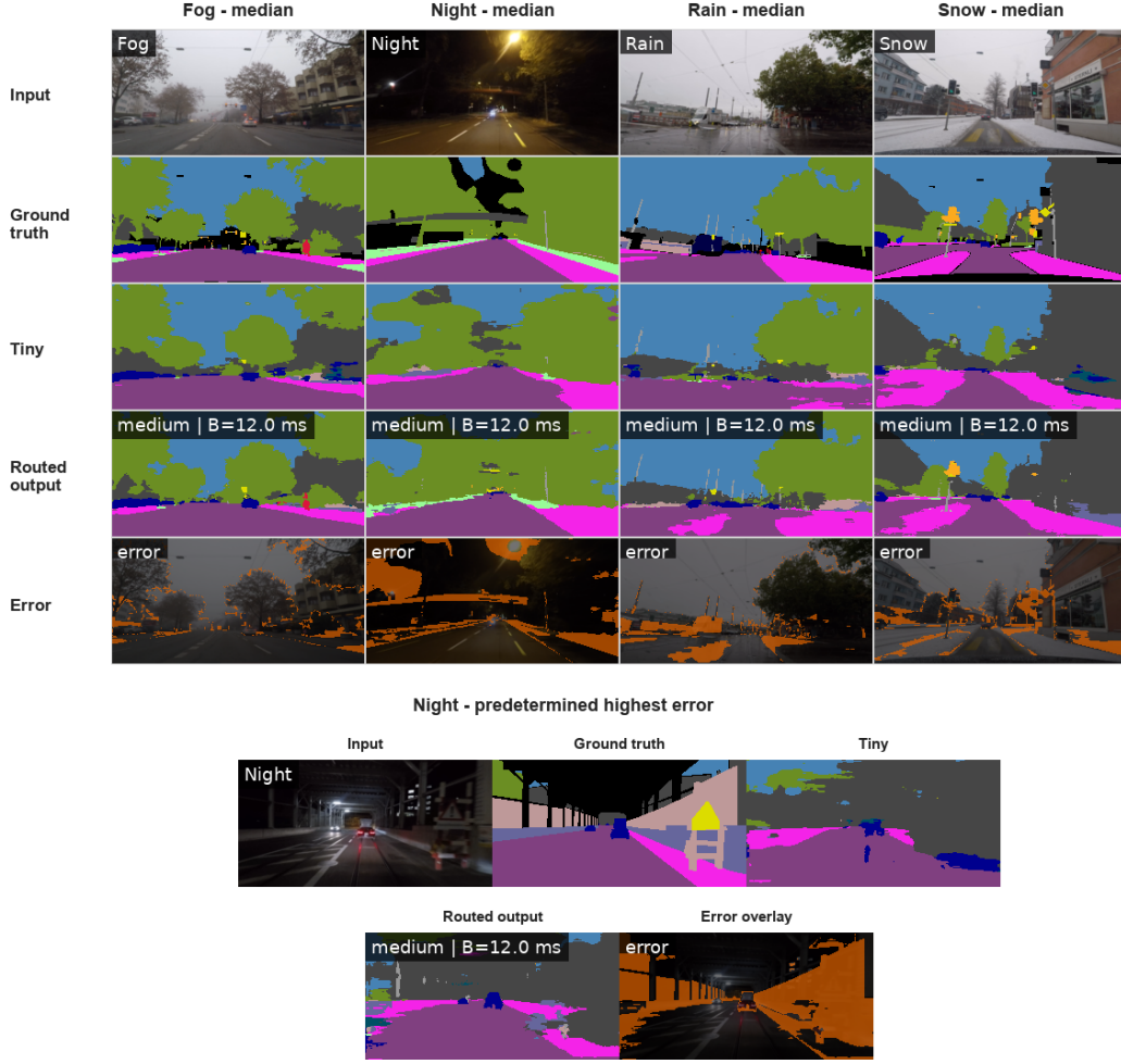
Figure S1: ACDC error gallery. The upper block contains deterministic median-error examples for fog, night, rain, and snow; the lower block enlarges the predetermined highest-error Run A ACDC case. Rows compare input, ground truth, tiny, routed output, and error. Orange marks disagreement with ground truth; the gallery does not estimate a failure rate.
