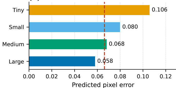
(b) Candidate risk · \tau=0.066
