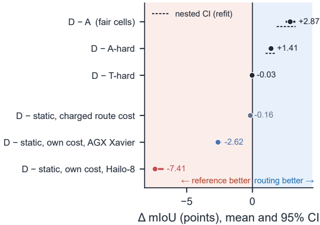
Figure 7: Routing gains come from the hard budget, not from candidate-specific calibration, and vanish against static deployment charged its own latency. Mean mIoU difference of policy D against each reference with image-level 95% bootstrap intervals (solid) and nested intervals that refit calibrators and operating points (dashed, where computed); median cost tables, 120 cells except the 62 fair cells of D – A.
