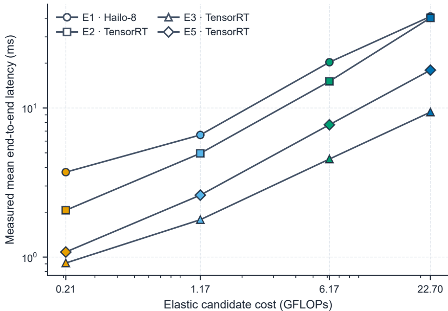
(a) Measured latency is hardware specific
