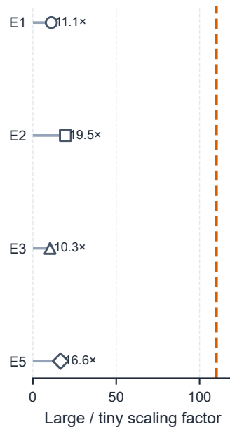
(b) FLOPs exaggerates scaling
