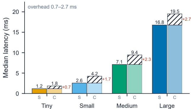
static deployment S_h (left) | route through tiny probe C_h (right) routing overhead C_h - S_h AGX Xavier (TensorRT FP16) Hailo-8 (INT8)
