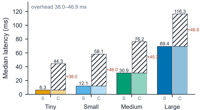
static deployment S_h (left) | route through tiny probe C_h (right) routing overhead C_h - S_h AGX Xavier (TensorRT FP16) Hailo-8 (INT8)
