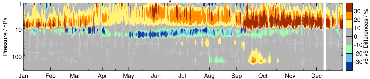
CH 3 CN at 0°
