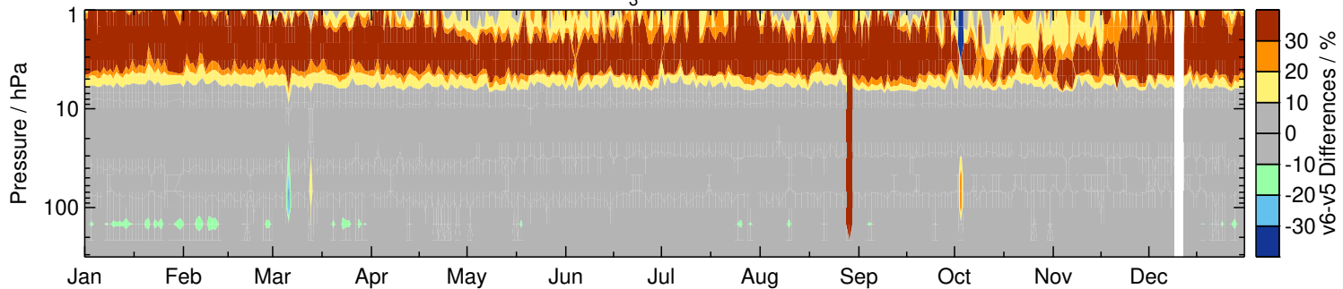
CH 3 CN at 75°N
