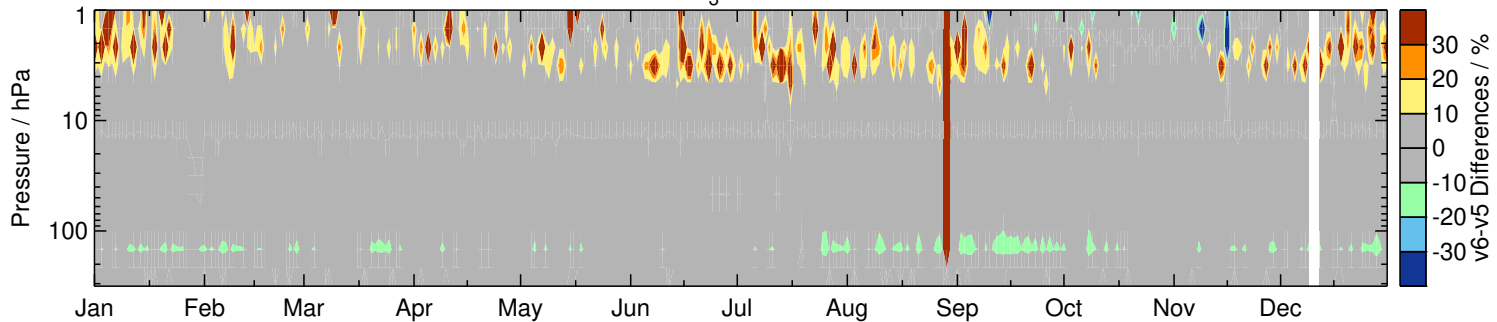
\text{CH}_3\text{Cl} at 75°N
