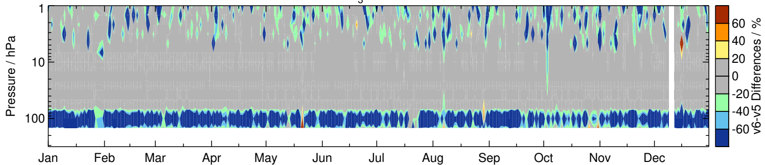
CH 3 OH at 75°N
