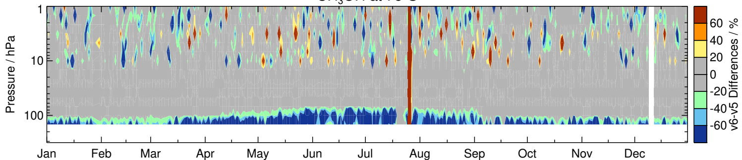
CH 3 OH at 0°
