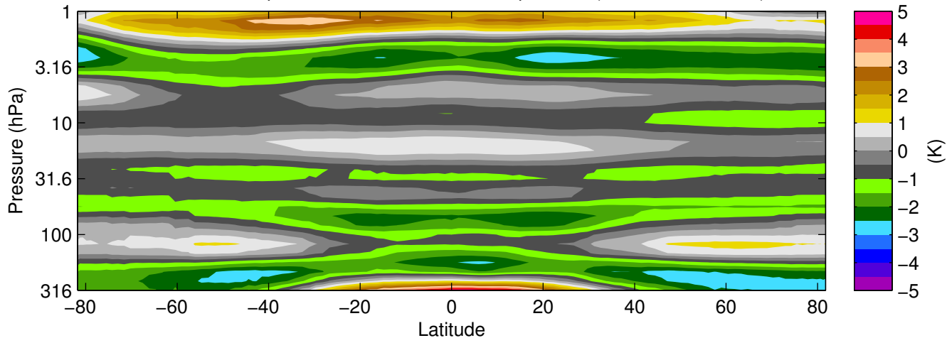
MLS v3.3 Temperature minus GEOS-5 Temperature (2005--2010 mean)
