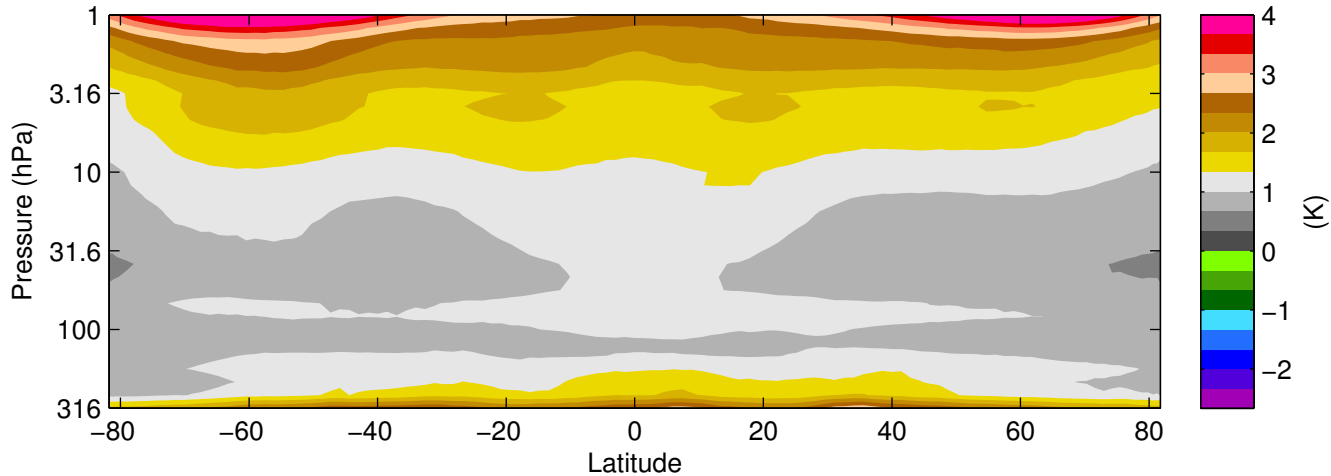
Standard Deviation of MLS v3.3 Temperature minus GEOS-5 Temperature (2005--2010)
