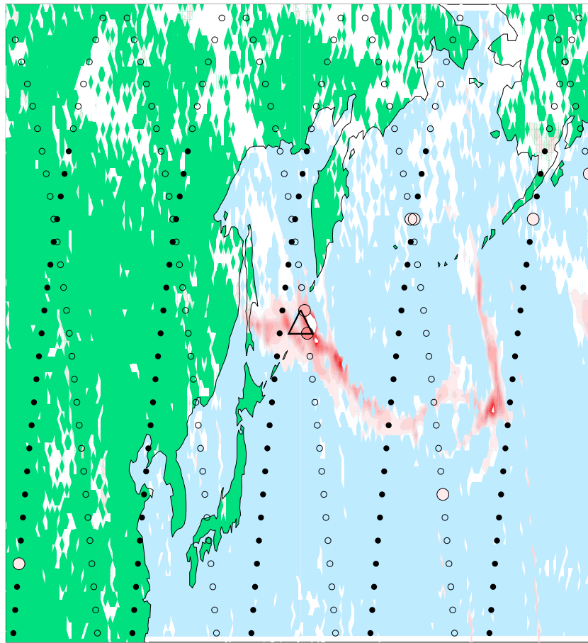
OMI SO2 column map of sarychev 2009.06.14
