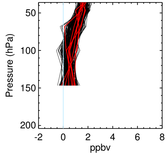
MLS HCl
