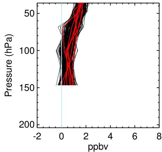
MLS HCl
