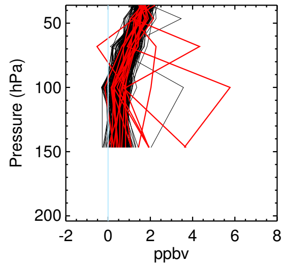
MLS HCl
