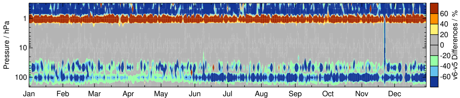
CIO at 75°N
