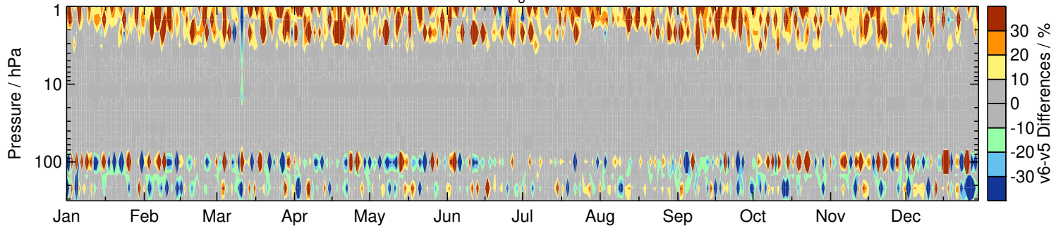
\text{HNO}_3 at 75°N
