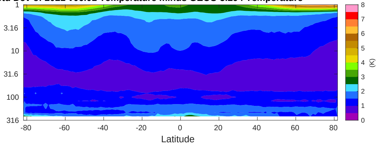
Std Dev of 2021 v06.01 Temperature minus GEOS-5.294 Temperature
