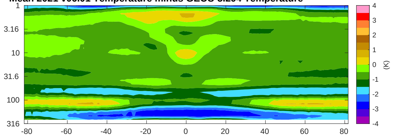
Mean 2021 v06.01 Temperature minus GEOS-5.294 Temperature
