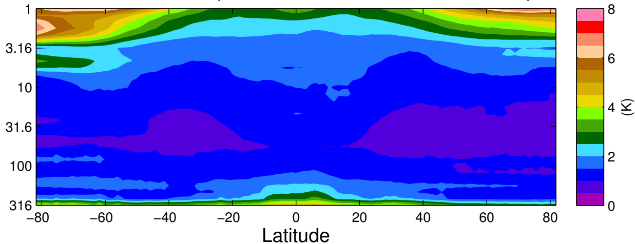
Std Dev of v04.20 Temperature minus GEOS-5.9 Temperature
