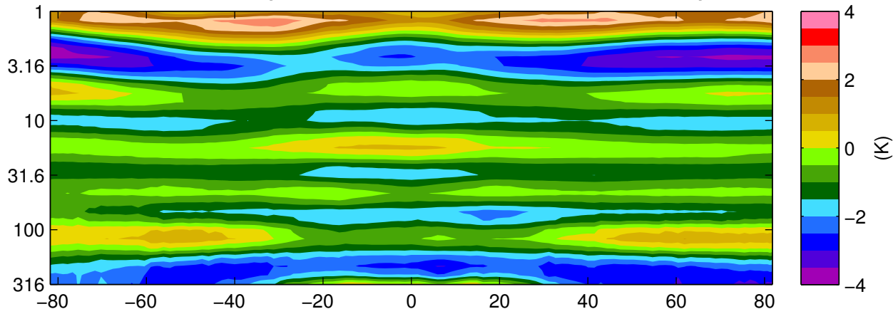
Mean v04.20 Temperature minus GEOS-5.9 Temperature
