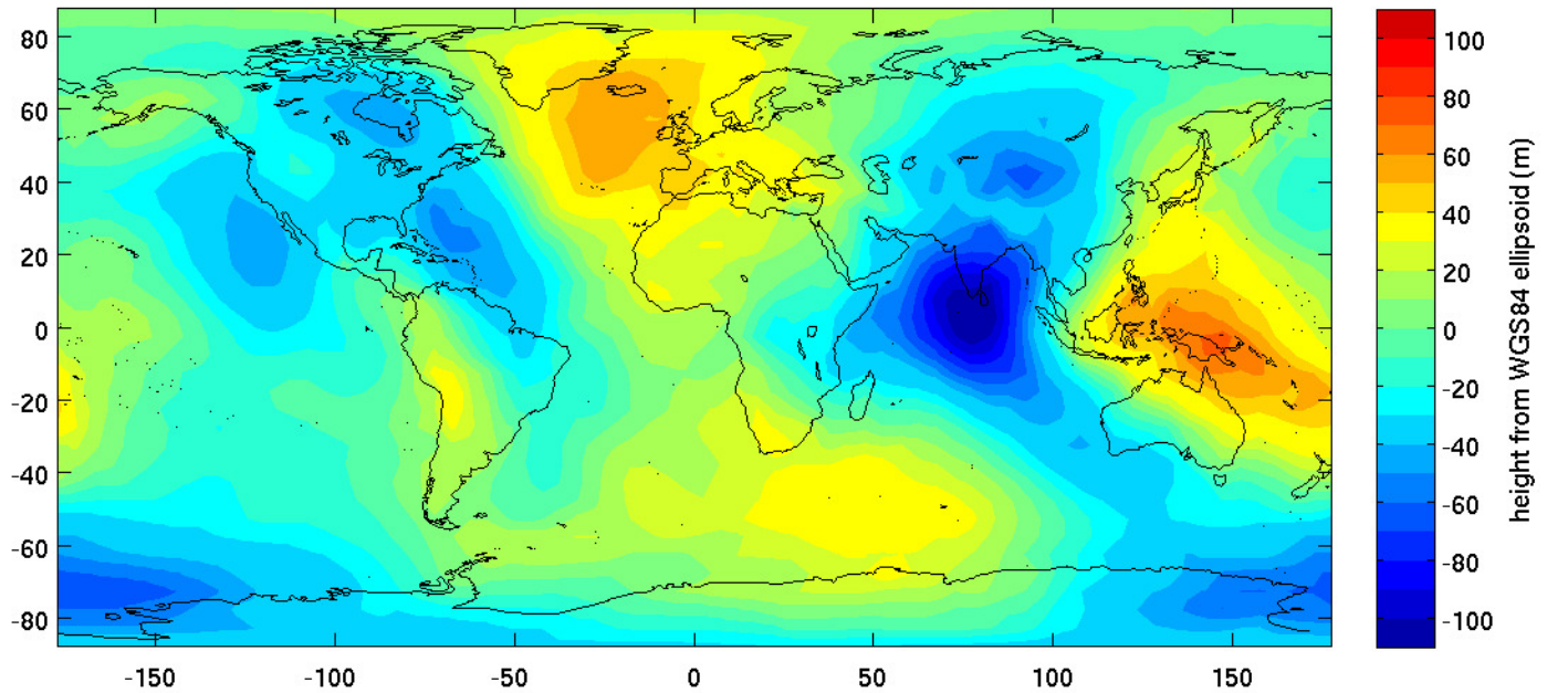
WGS84 EGM96 Geoid
