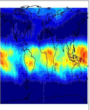
MLS V04.20
