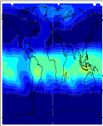
AIRS V6
