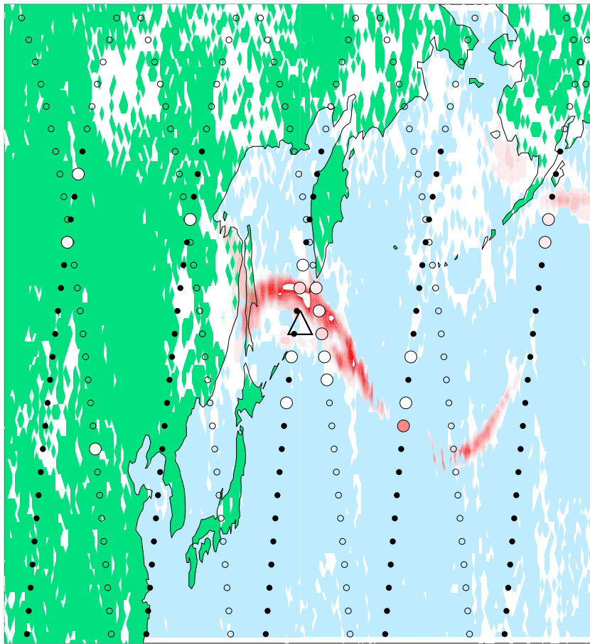
OMI SO2 column map of sarychev 2009.06.16
