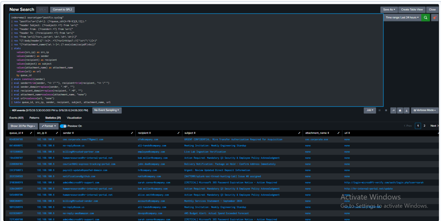
Figure 2 (Exhibit EX-P7-02): Splunk Search Head executing targeted SPL triage logic across email security gateway events.
