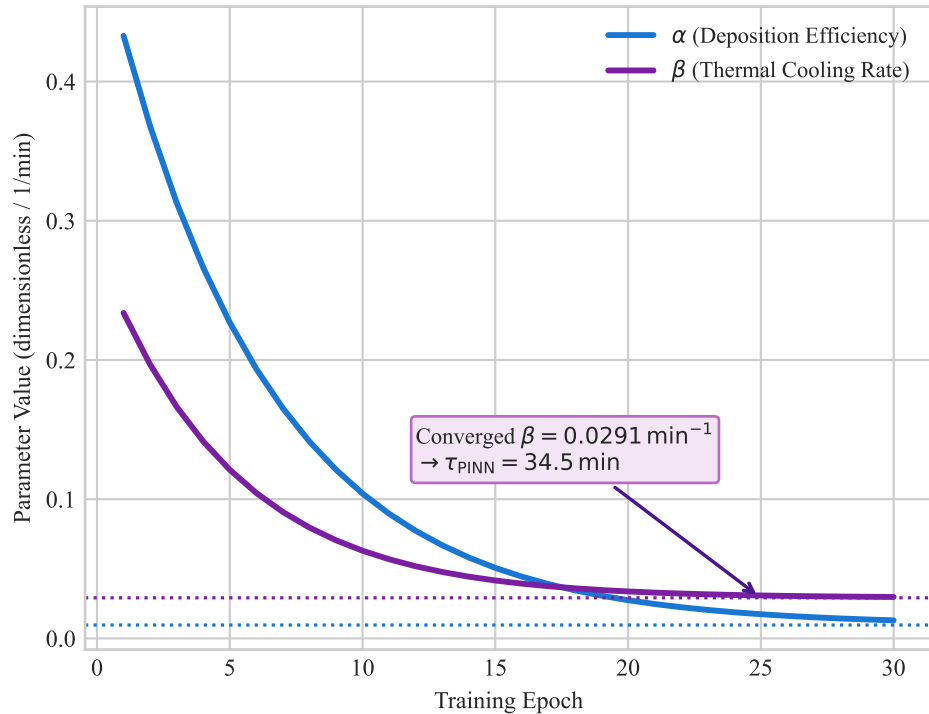
(a) Convergence of PINN Parameters \alpha and \beta
