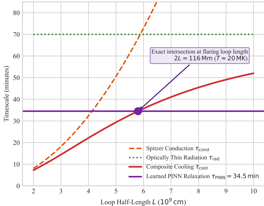
(b) Coronal Cooling Timescales vs. PINN \tau_{\text{PINN}} = 34.5 \text{ min}
