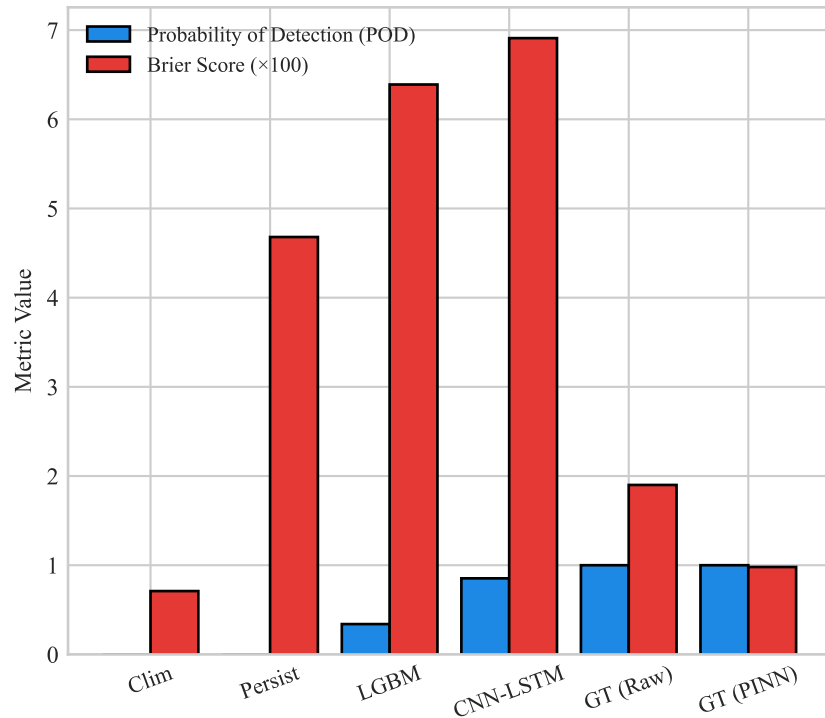
(b) Precursor Sensitivity (POD) and False Alarm Penalty
