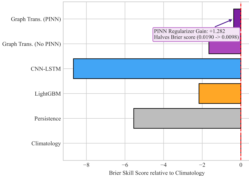
(a) Probabilistic Calibration: Brier Skill Score (BSS)
