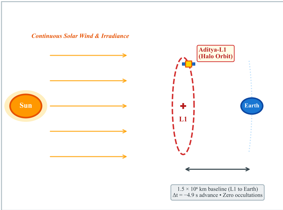
(a) Aditya-L1 Halo Orbit at Sun-Earth Lagrangian Point L1
