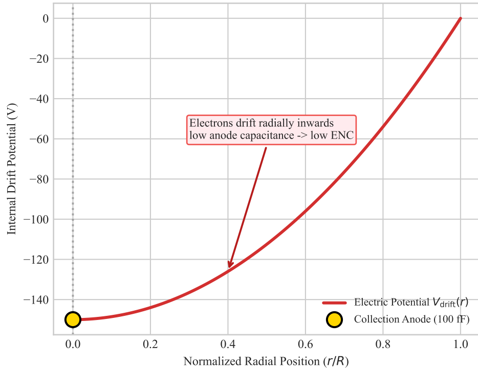
(a) SoLEXS: Silicon Drift Detector (SDD) Radial Field
