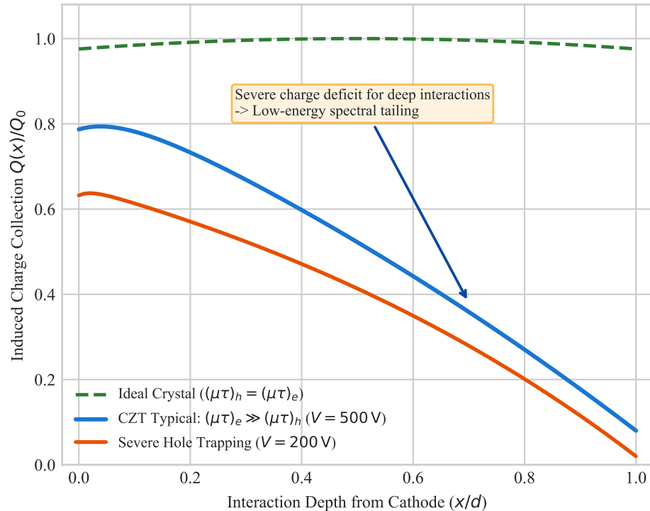
(b) HEL10S CZT: Depth Charge Collection & Hecht Equation
