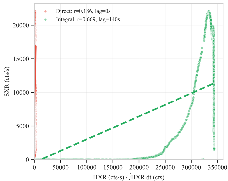
20241003 - X9.0
