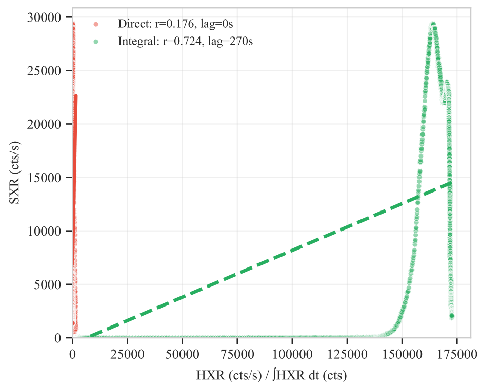
20240514 - X8.7
