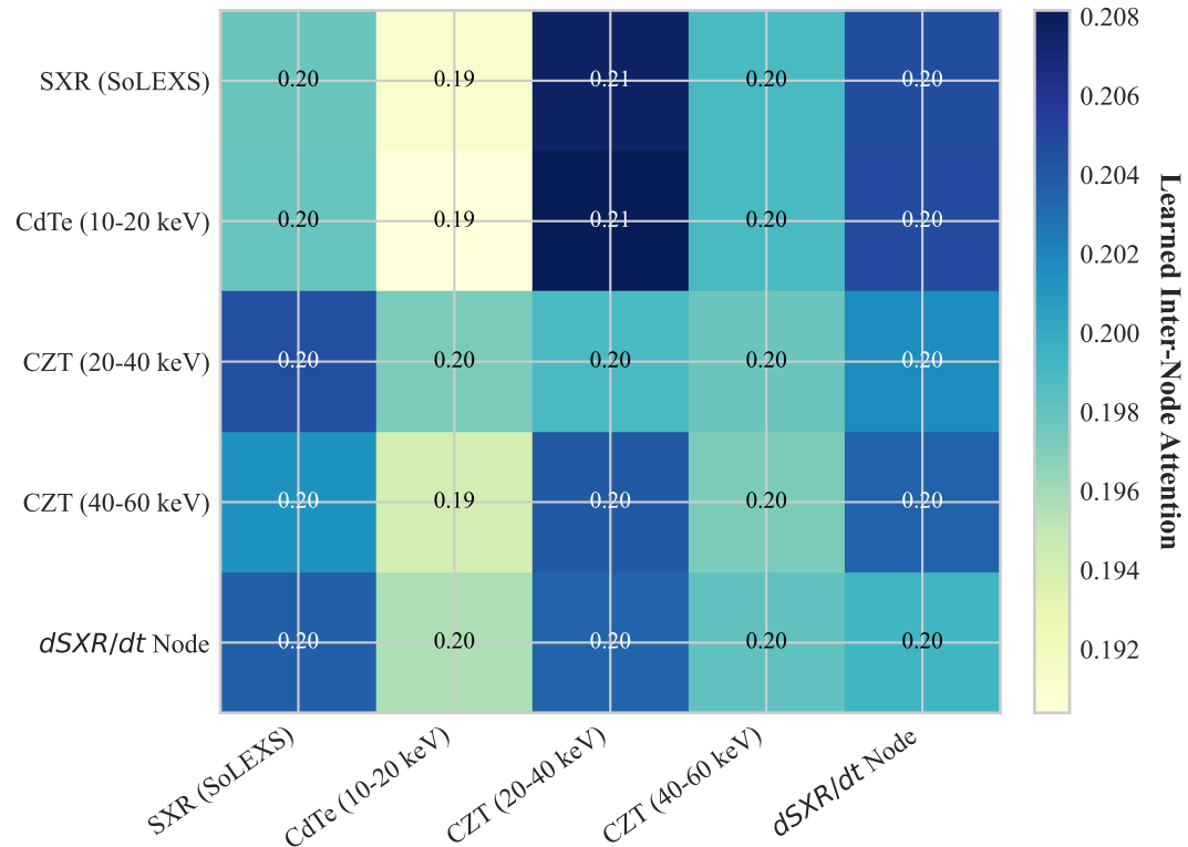
(b) Multi-Detector Spatial Graph Coupling
