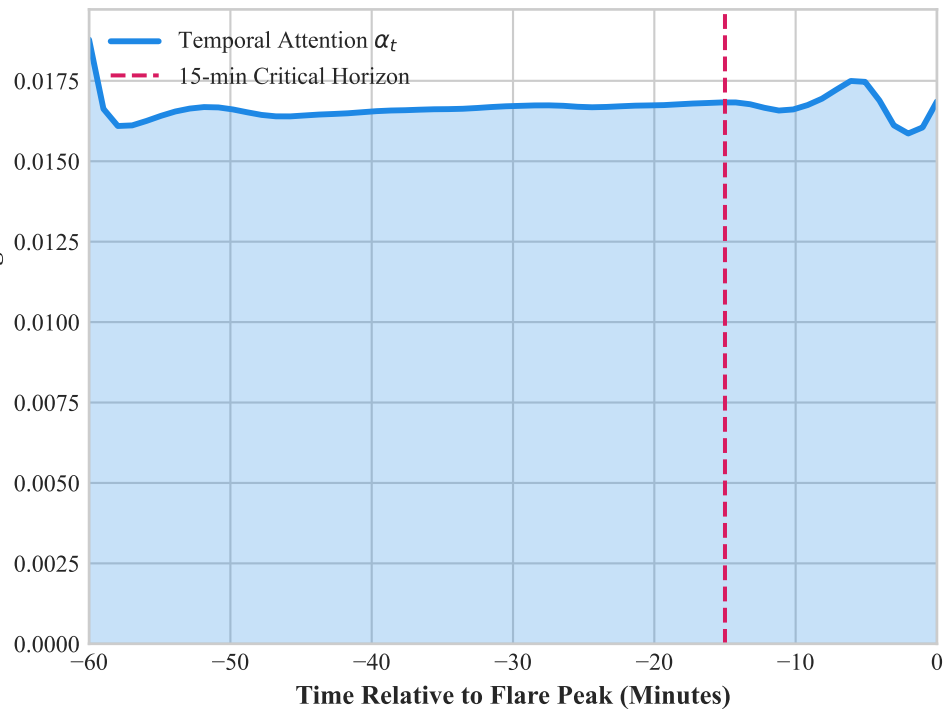
(a) Precursor Temporal Attention Distribution
