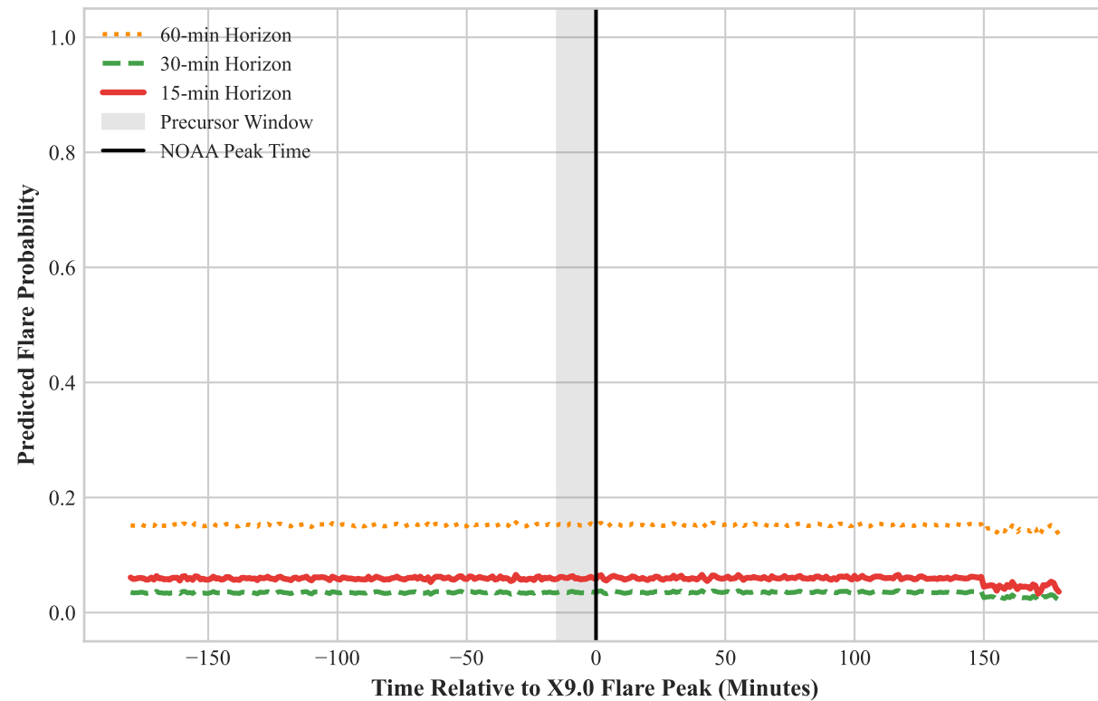
(a) Multi-Horizon Probability Trajectories (X9.0 Flare)
