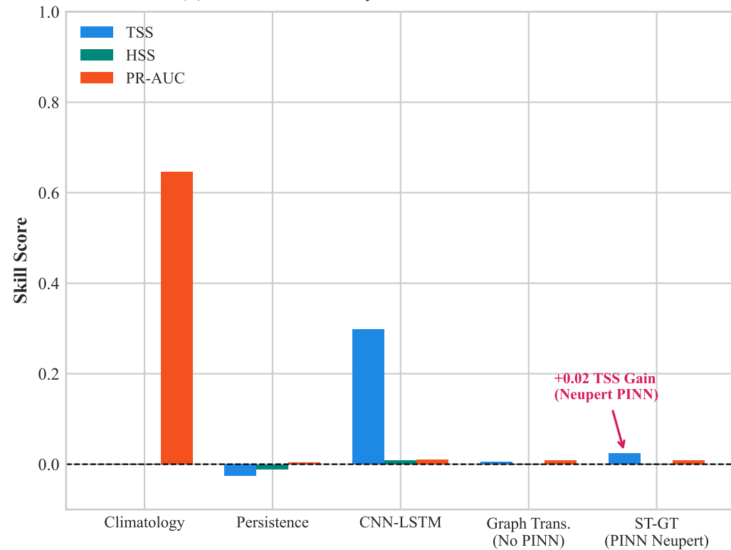
(b) Model Skill & Physics Inductive Bias Ablation
