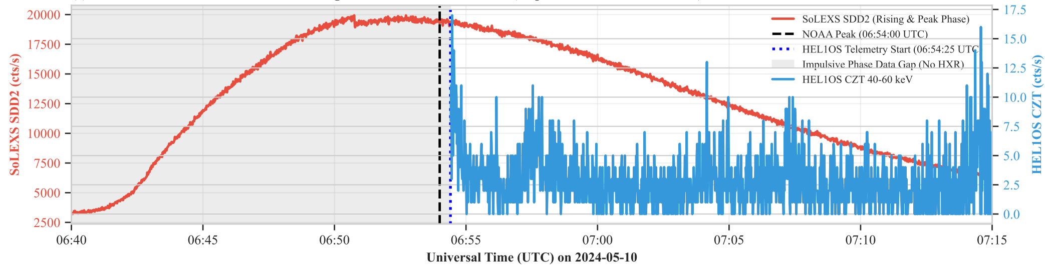
(c) Zoom Around X3.9 Peak: HEL10S Begins +25s After NOAA Peak (Impulsive Phase Unobserved)
