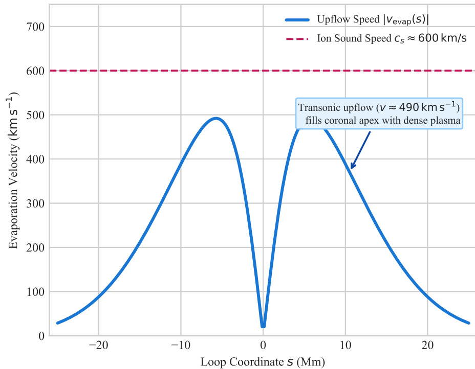
(b) Explosive Evaporation Upflow Velocity v_{\text{evap}}(s)
