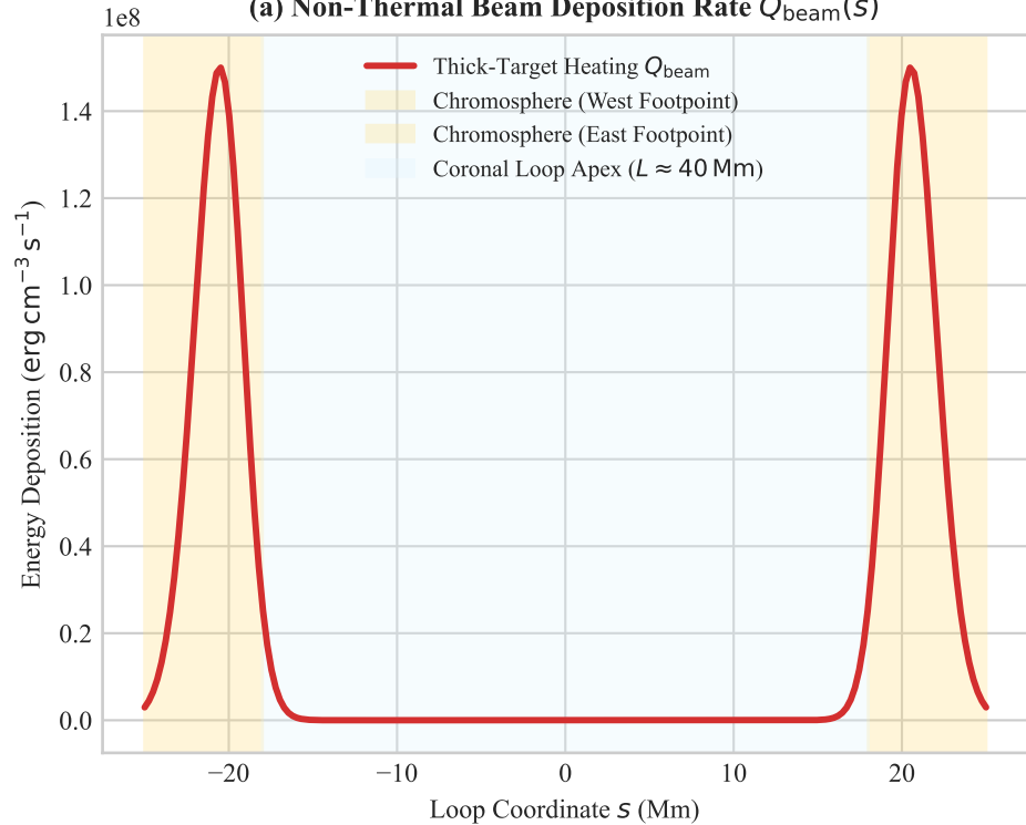
(a) Non-Thermal Beam Deposition Rate Q_{\text{beam}}(s)
