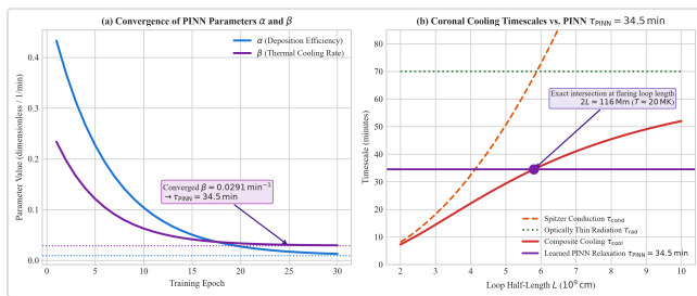
Figure 10. Physics verification of the PINN inductive bias. (a) Convergence of learned parameters \alpha(t) and \beta(t) during training, reaching steady-state \beta = 0.0291 \text{ min}^{-1} ( \tau_{\text{PINN}} = 34.5 \text{ min} ). (b) Theoretical Spitzer conductive ( \tau_{\text{cond}} ) and CHIANTI radiative ( \tau_{\text{rad}} ) cooling curves vs loop length L . The learned relaxation time matches the physical composite cooling time \tau_{\text{cool}} at 2L \approx 116 \text{ Mm} for T_e = 20 \text{ MK} .
