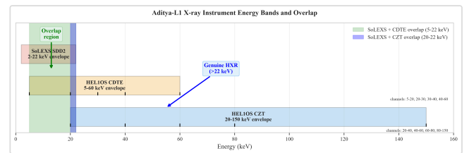
Figure 3. In-flight energy band envelopes and channel boundaries extracted directly from Level-1 FITS EXTNAME headers. The only genuine HXR channels available to this study lie strictly above the 22 keV SoLEXS ceiling.
