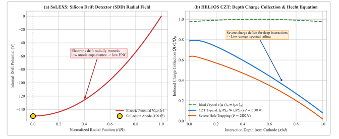
Figure 2. Microscopic semiconductor detector physics. (a) SoLEXS Silicon Drift Detector (SDD): radial drift electric potential V_{drift}(r) guiding electron clouds to the low-capacitance central collection anode pin ( C_{anode} \sim 100 fF). (b) HELIOS CZT: hole-trapping depth-dependent charge collection fraction Q(x)/Q_0 modeled via the Hecht equation for different mobility-lifetime ratios (\mu\tau)_h , illustrating low-energy spectral tailing.
