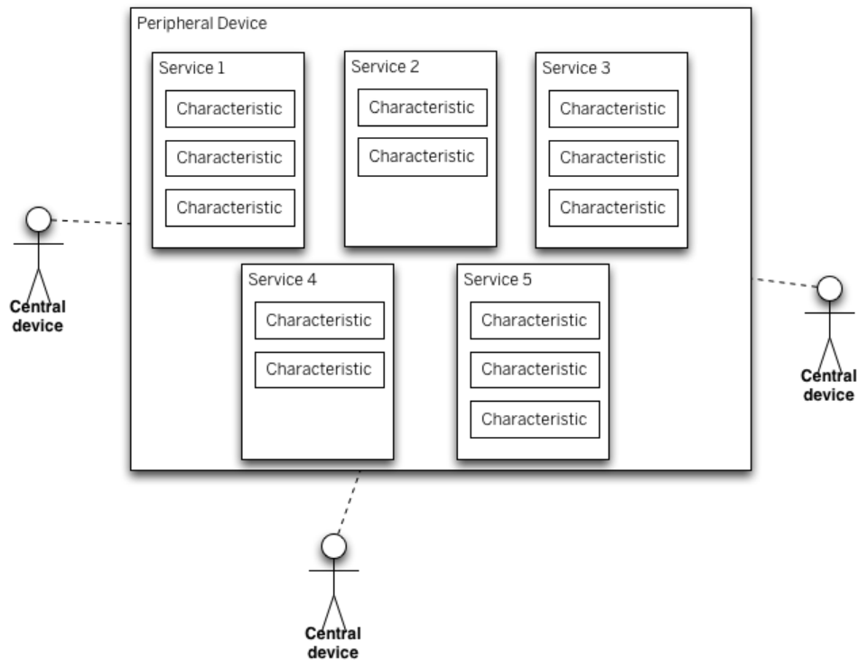
Figure 10.6.: BLE Devices – Peripheral and Central Devices
