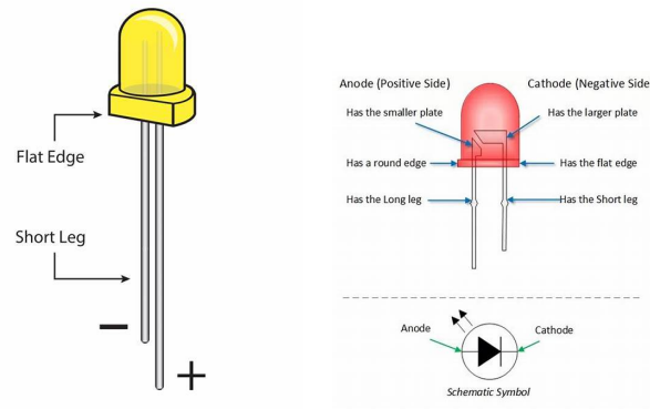
Figure 12.2.: Parts of a LED.
