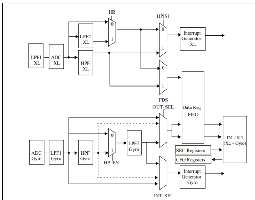
Figure 11.10.: Accelerometer and gyroscope block diagram [Stmb]
